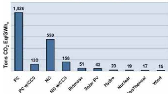
Figure 6.10: Comparison of CO 2 Emissions for Electricity Generating Technologies
