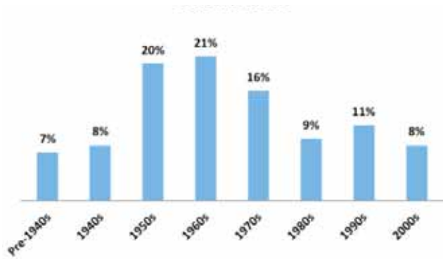
Figure 5.6: Hazardous Liquid Pipelines by Period of Construction
