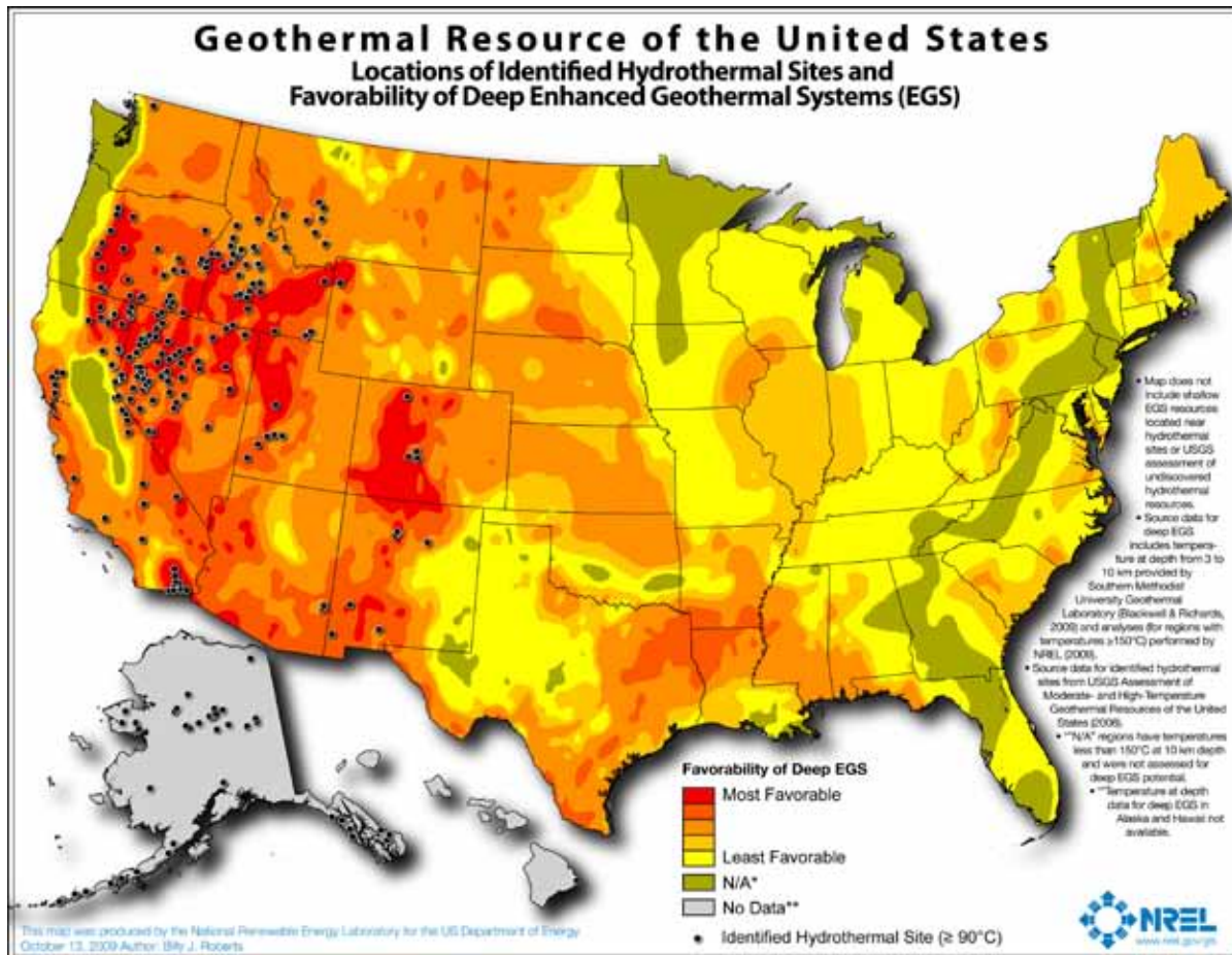
Figure 1.17: Geothermal Resources of the Western States
