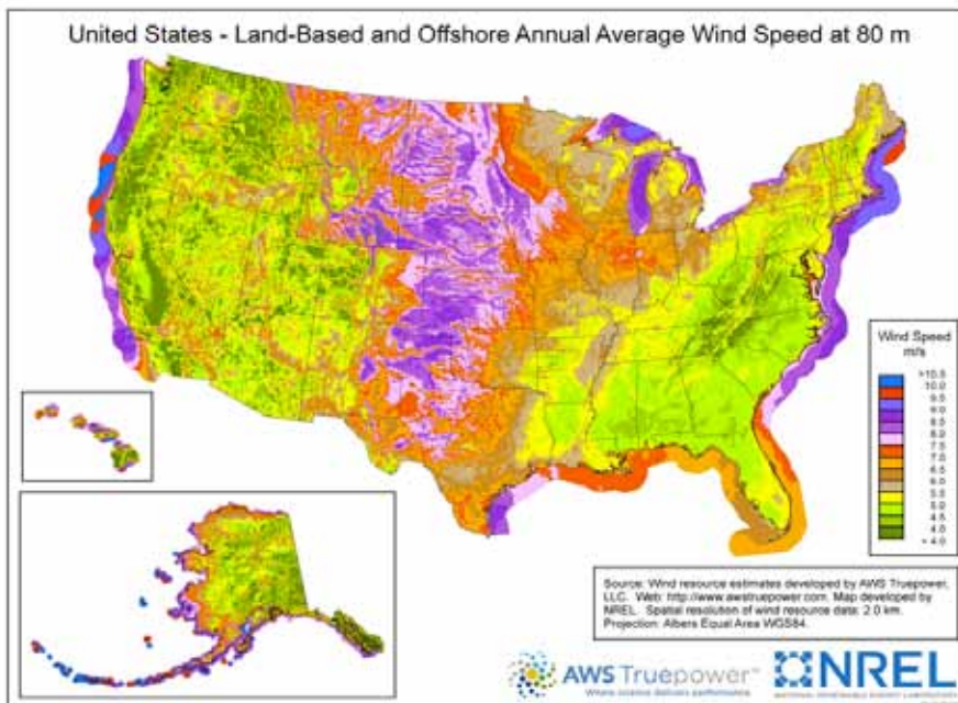
Figure 1.11: U.S. Wind Power Resource at 80 meters
