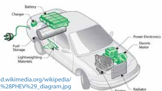
Figure 3.3: Plug-in Hybrid Electric Vehicle (PHEV)
